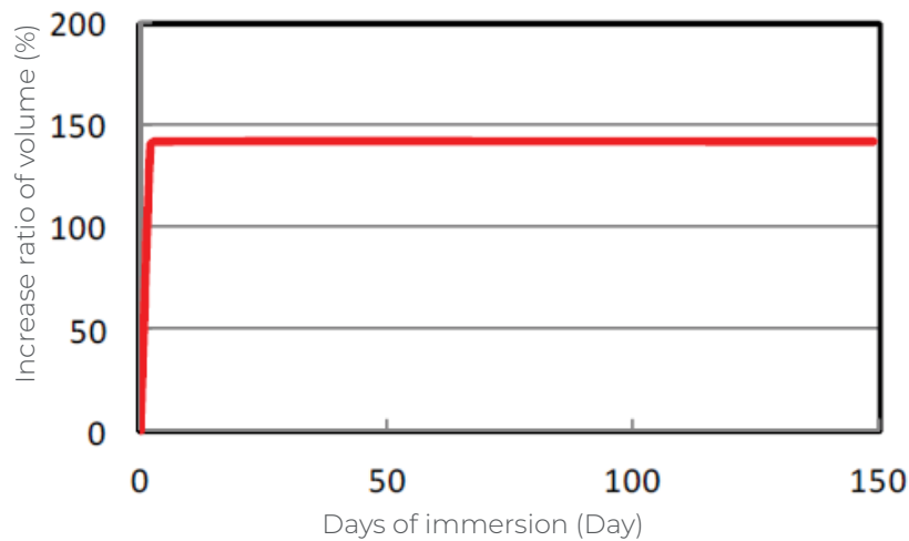
Figure 2 : Long term swelling characteristics of Leakmaster in Distilled water
