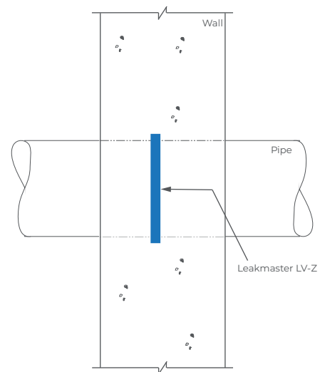
Application of Leakmaster around pipe penetration through wall (cast-in-situ method). The same application can be applied for slab areas.
