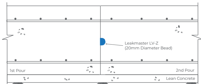
Application of Leakmaster in Construction Joint of Wall or Slab
