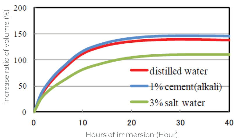
Figure 1: Swelling properties in various solutions of Leakmaster
